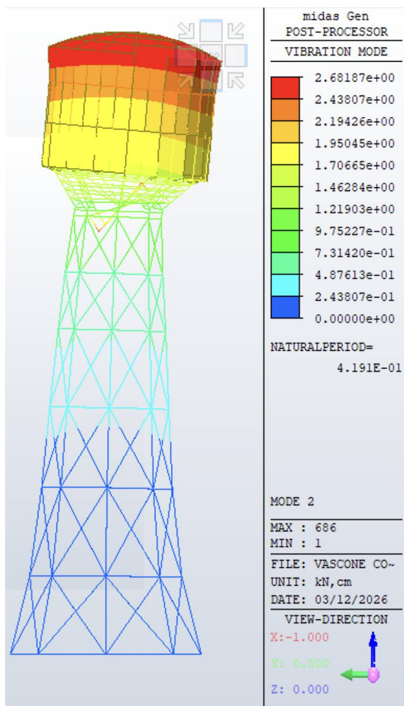
Figura 7 - ModeShape2
